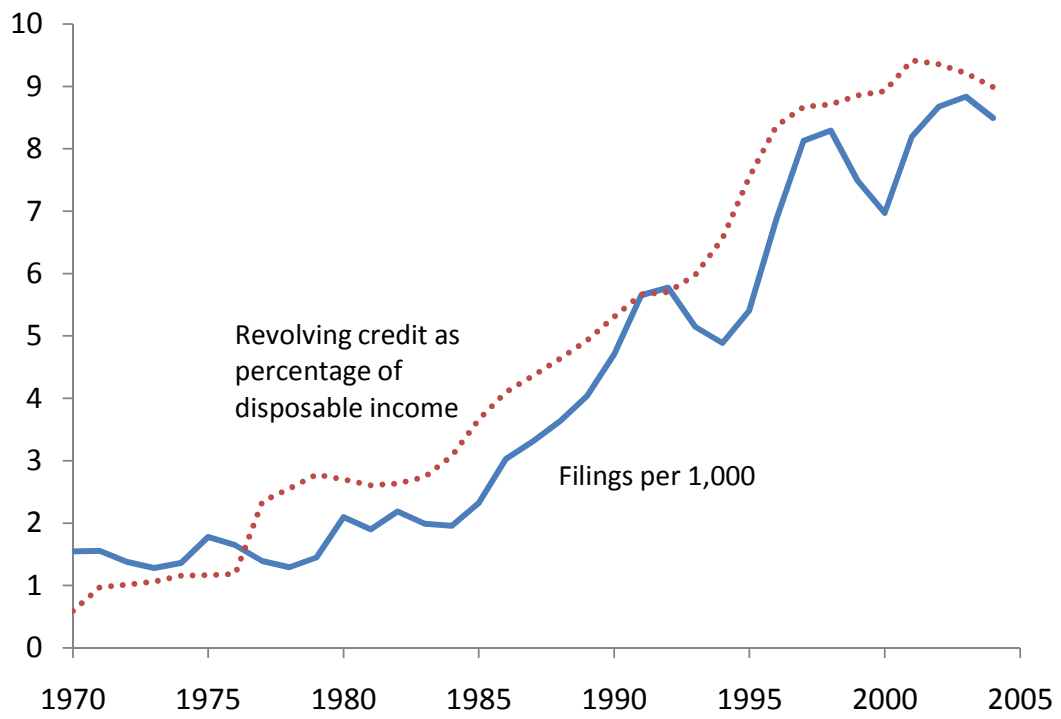
Figure 1: Aggregate Facts
